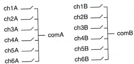
Figure 3. PXI-2596 Power-On State
