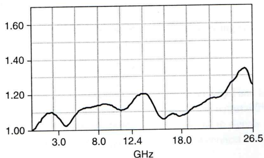
Figure 2. VSWR, Typical
