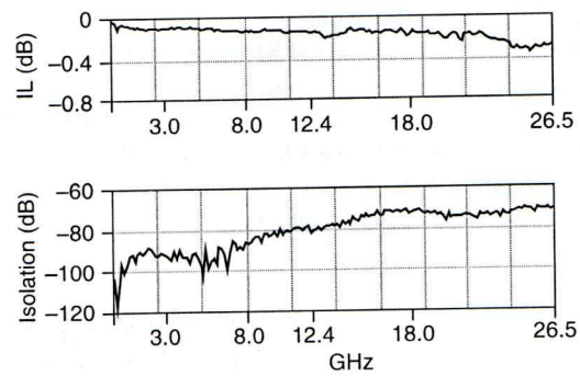
Figure 1. Insertion Loss and Isolation, Typical
