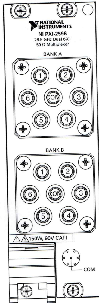
Figure 4. PXI-2596 Front Panel
